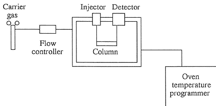
Figure 9.2 Schematic diagram of GC
